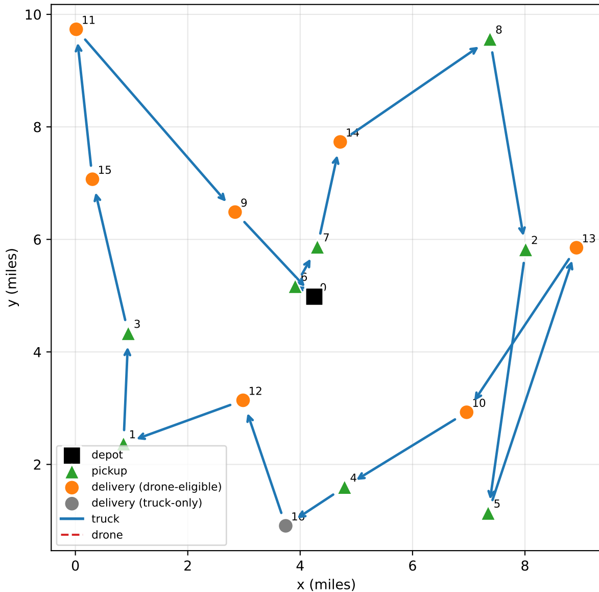
V6 truck-only baseline (16.10.3) z = $4.316
